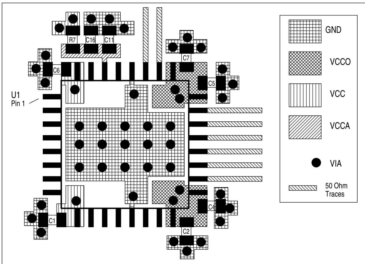
FIGURE 5B. PCB BOARD LAYOUT FOR ICS8735-01
