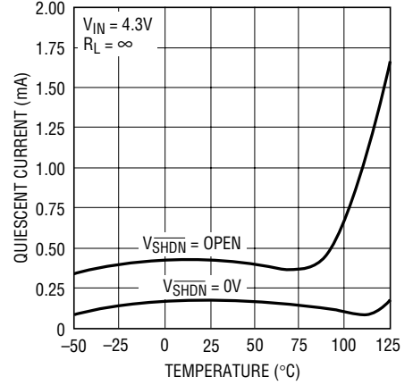
Quiescent Current
