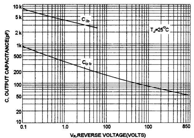
FIG-7 CAPACITANCES
