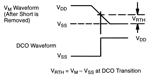
FIGURE 3. Reset Threshold
