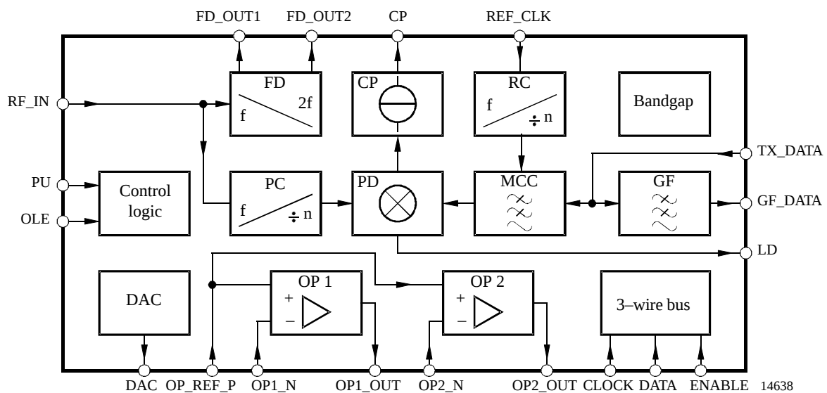
Figure 1. Block diagram
