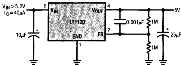
5V Regulator
