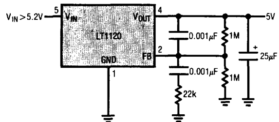
Regulator with Improved Transient Response
