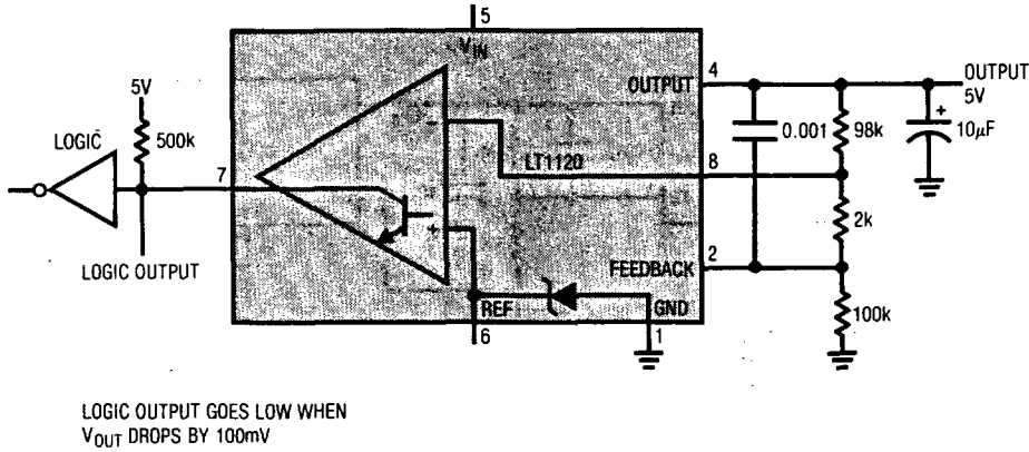
Regulator with Output Voltage Monitor
