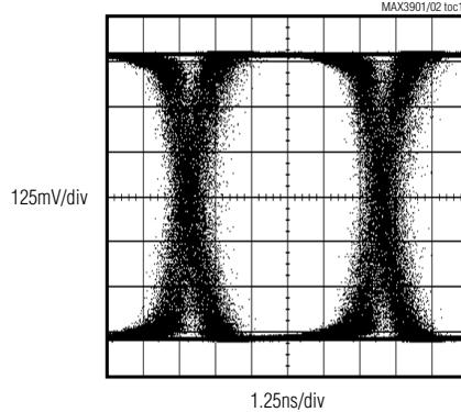
OUTPUT EYE DIAGRAM (-27.7dBm OMA OPTICAL INPUT AT T J = +25°C) SILICON PHOTODIODE WITH 850nm SOURCE
