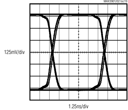
OUTPUT EYE DIAGRAM (+3dBm OMA OPTICAL INPUT AT T J = +25°C) SILICON PHOTODIODE WITH 850nm SOURCE
