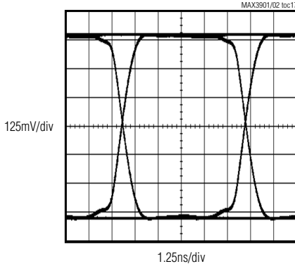
OUTPUT EYE DIAGRAM (1mAp-p ELECTRICAL INPUT AT T J = +25°C)
