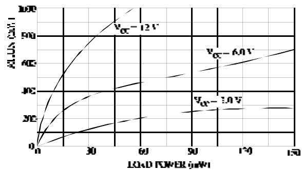
Figure 2. DEVICE DISSIPATION 8.0 W LOAD
