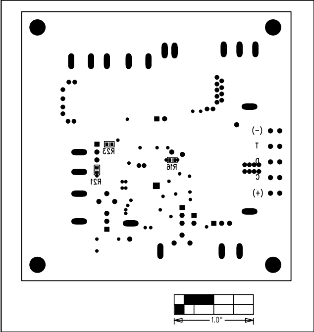
Figure 7. MAX8724 EV Kit PC Board Layout—Solder Side
