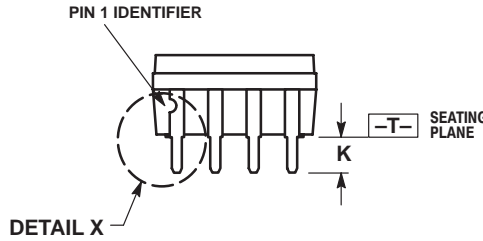
CASE 482B-03 ISSUE B
