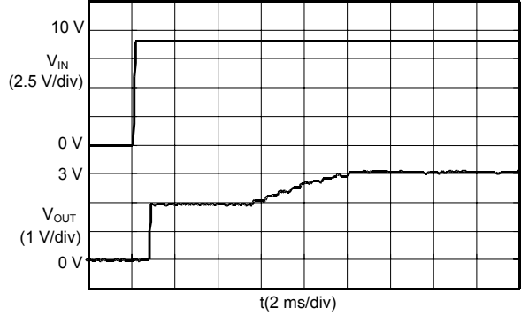
S-8520/1C30MC ( V_{IN} : 0 → 9.0 V)
