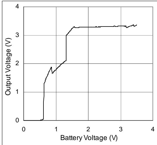
Figure 4. V_{OUT} vs. V_{BATT} ; Shutdown, 300mA Load
