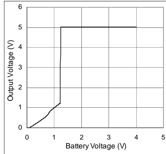
Figure 17. V_{OUT} vs. V_{BATT} ; Shutdown, No Load
