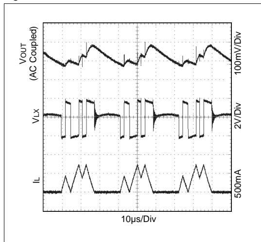
Figure 12. Waveforms; R_{LOAD} = 33\Omega
