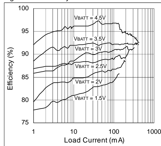
Figure 25. Efficiency vs. Load Current
