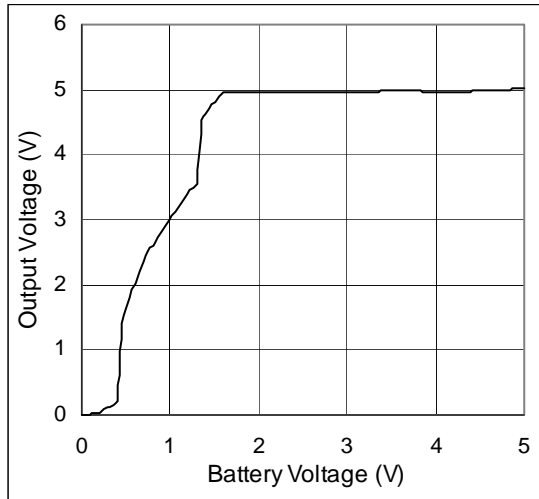
Figure 16. V_{OUT} vs. V_{BATT} ; Shutdown, 180mA Load
