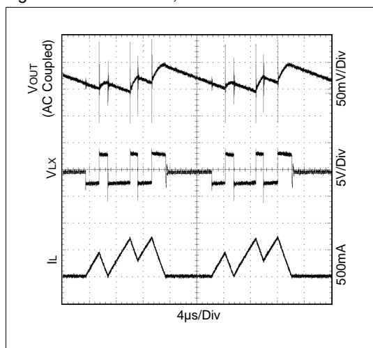
Figure 24. Waveforms; R_{LOAD} = 68\Omega
