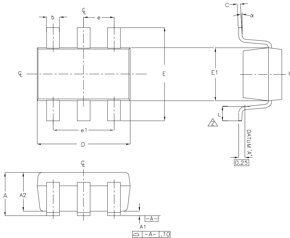
Figure 29. 6-pin SOT23 Package
