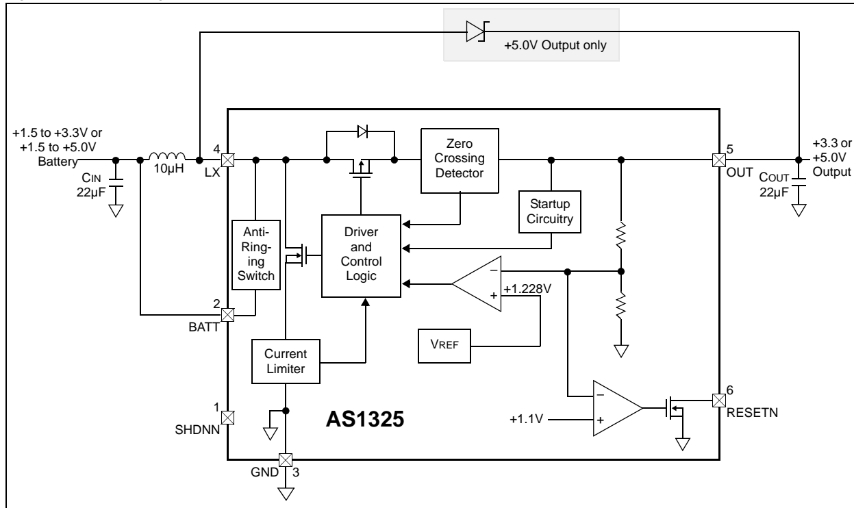
Figure 26. Block Diagram
