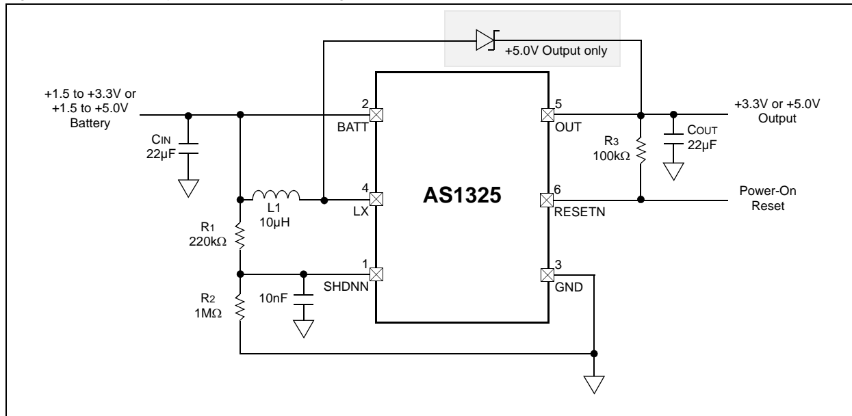
Figure 27. Low-Battery Cutoff Application Diagram
