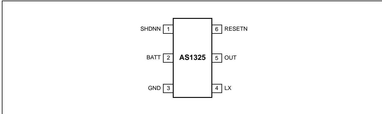
Figure 28. Pin Assignments (Top View)
