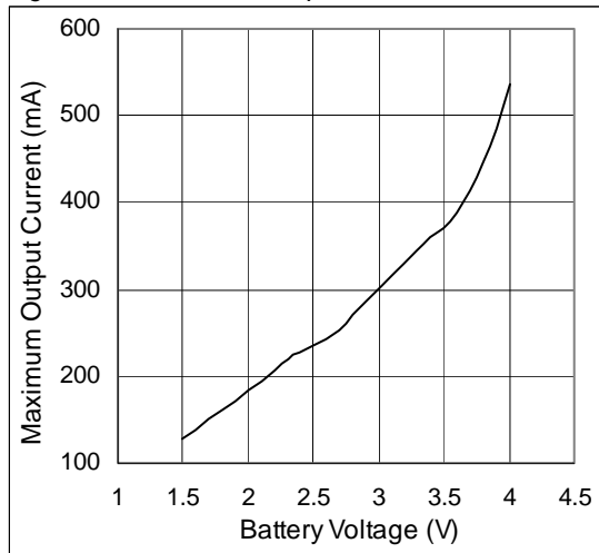
Figure 18. Maximum Output Current vs. V_{BATT}
