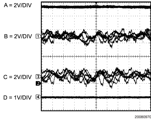
FIGURE 10. Same conditions and waveforms as shown in Figure 8, except that a 4700 \mu F capacitor has been connected between the V_{DD} pin and GND (Trace A)
