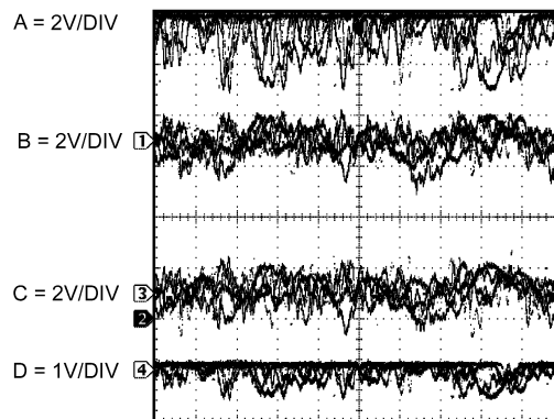
FIGURE 7. LM4952 operating on an unregulated 12\text{V} (nominal) power supply. Wave forms shown include V_{DD} (Trace A), V_{OUT A} (Trace B), V_{OUT B} (Trace C), and the DC voltage applied to the DC VOL pin (Trace D)
