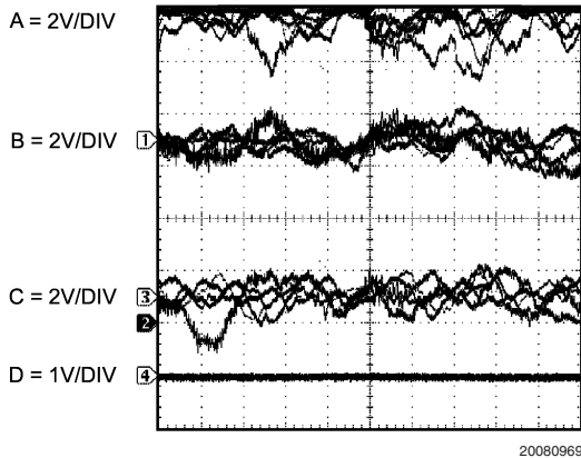
FIGURE 8. Same conditions and waveforms as shown in Figure 7, except that a 10 \mu F capacitor has been connected between the DC VOL pin and GND (Trace D)
