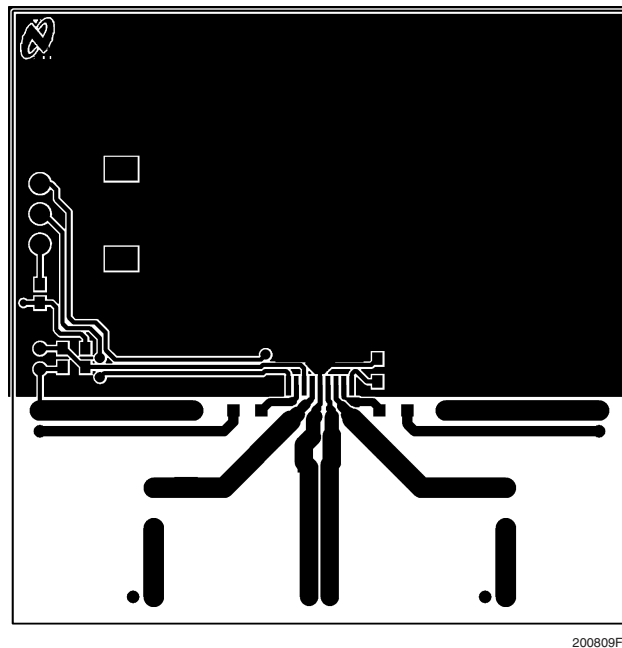
FIGURE 12. Recommended TS SE PCB Layout: Top Layer
