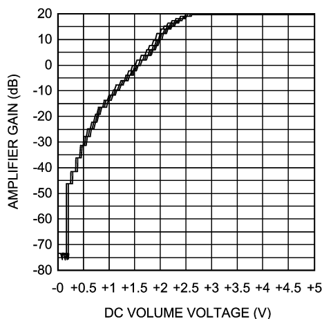
FIGURE 5. Typical part-to-part gain variation as a function of DC Vol control voltage
