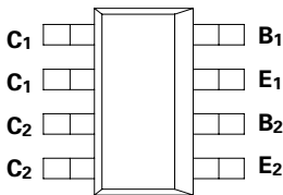
PARTMARKING DETAIL – ZDT1147
