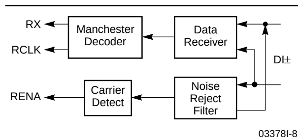
Figure 4. Receiver
