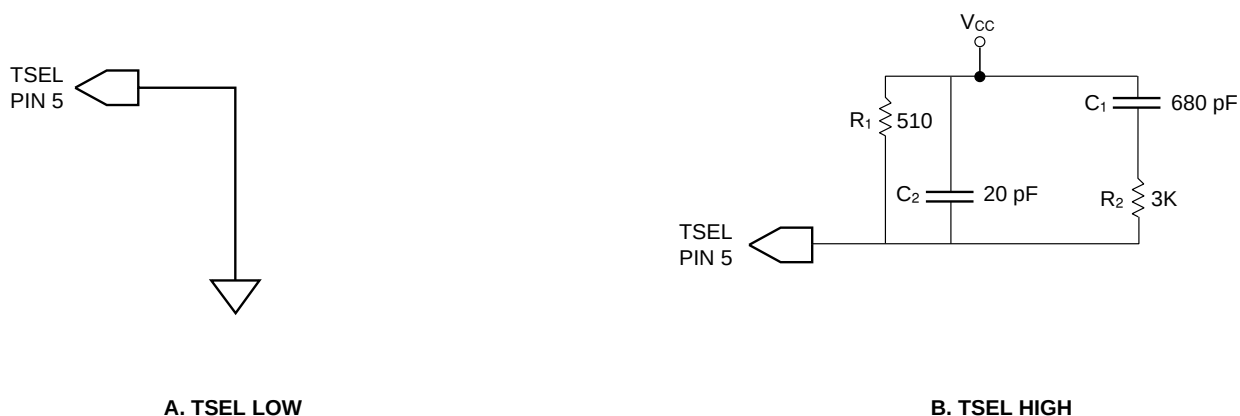
Figure 2. Transmitter Mode Select (TSEL) Connection
