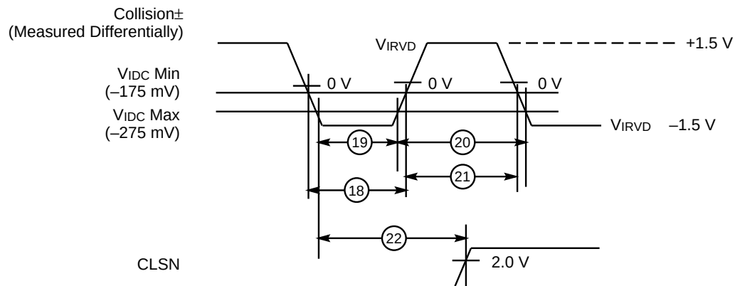
Collision \pm Input Pulse Width Timing
