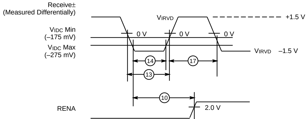
Receive \pm Input Pulse Width Timing
