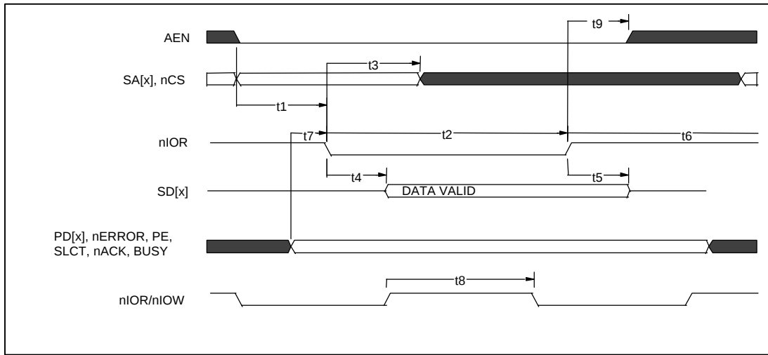
FIGURE 7 - ISA READ
