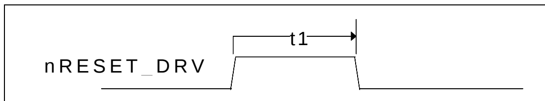
FIGURE 9C - RESET TIMING
