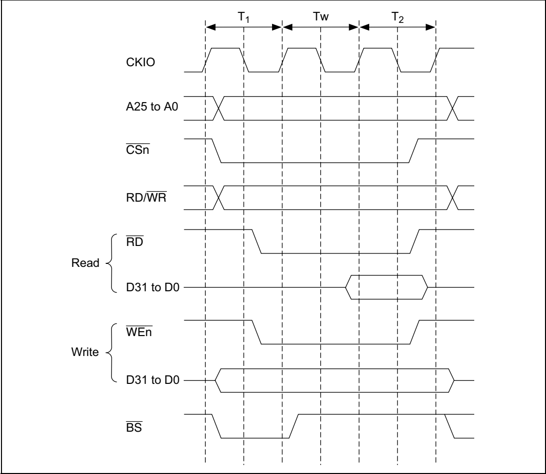
Figure 10.10 Basic Interface Wait Timing (Software Wait Only)
