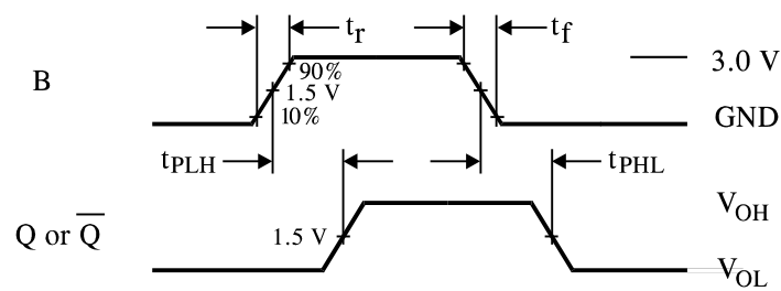
Figure 2. Switching Waveforms
