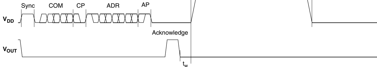
Fig. 5-4: Telegram for coding the EEPROM programming
