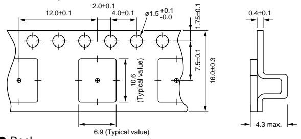
LDHA2 Series
