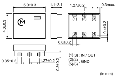
LDH54 Series
