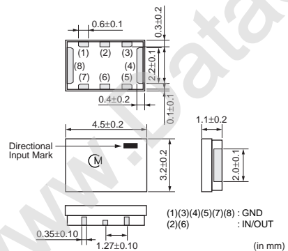
LDH43 Series
