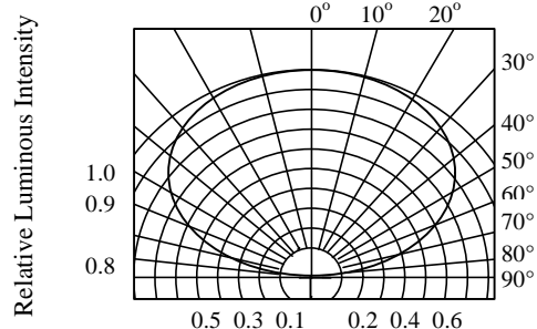
FIG.6 RADIATION DIAGRAM
