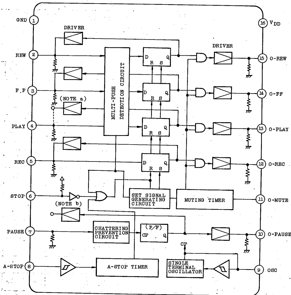
BLOCK DIAGRAM
