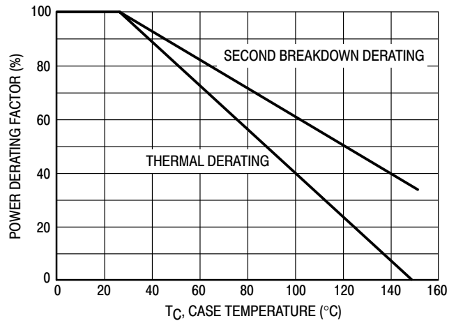
Figure 6. Power Derating
