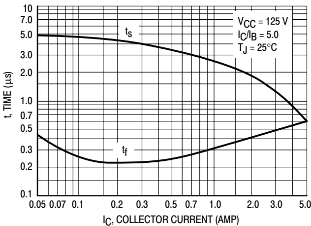
Figure 5. Turn-Off Time
