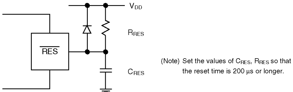
Figure 4 Reset Circuit
