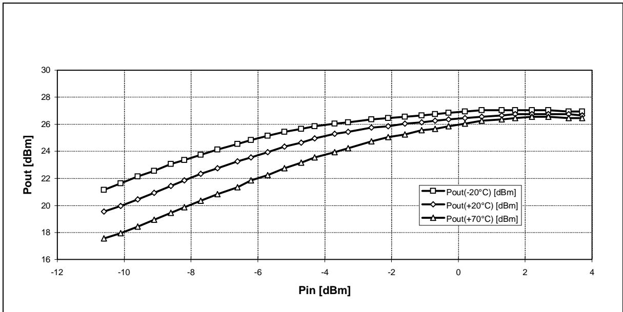
Output power at different temperatures*
