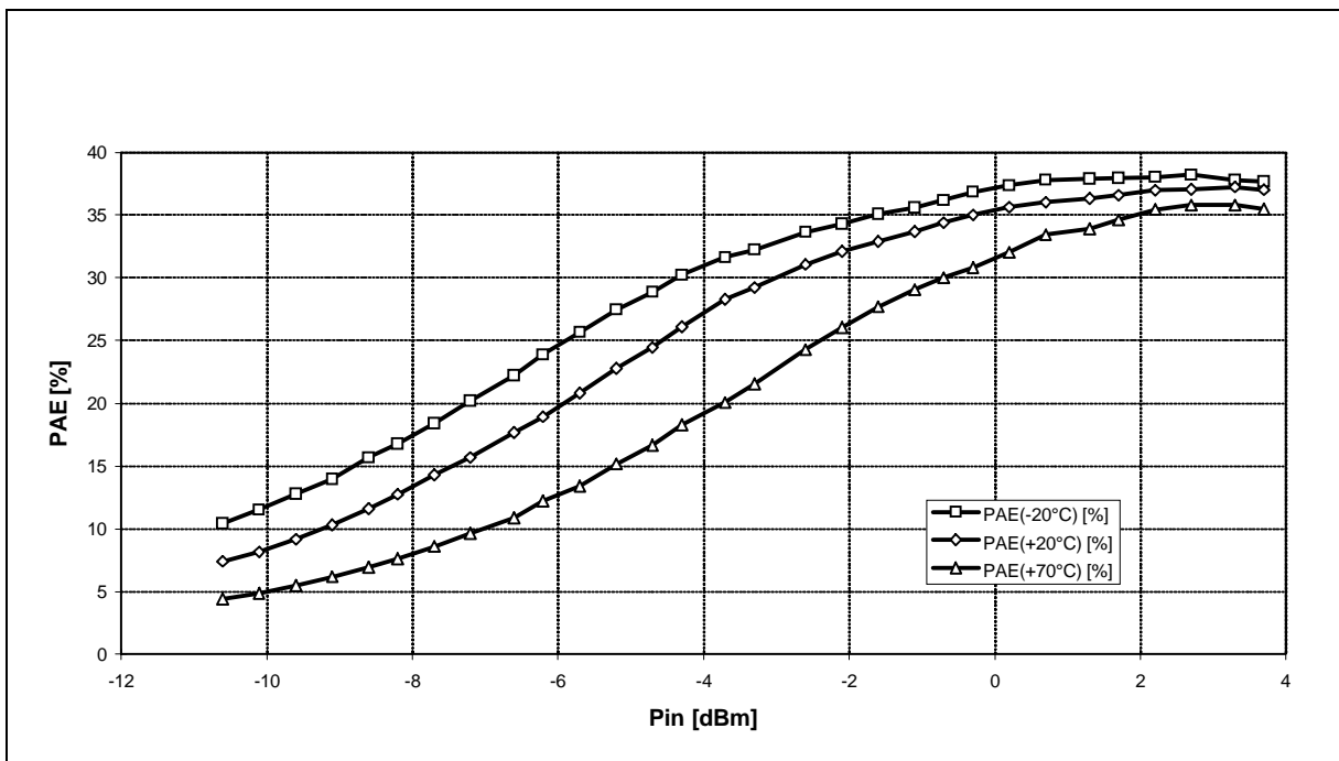
Power added efficiency at different temperatures*
