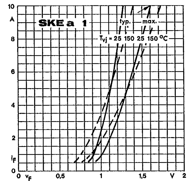
Fig. 6 a Forward characteristics
