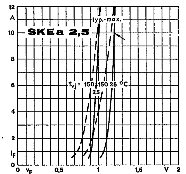
Fig. 6 c Forward characteristics
