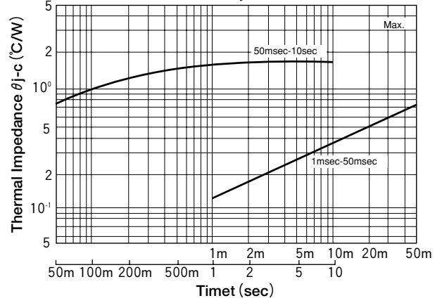
Transient Thermal Impedance (DIODE)
