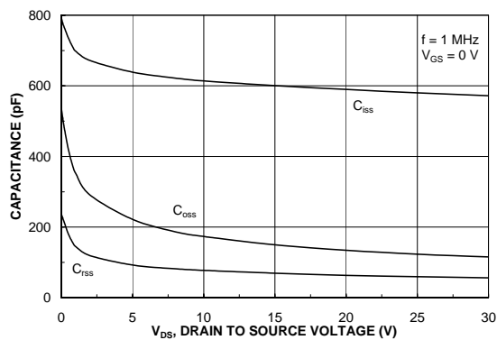
Figure 19. Capacitance Characteristics.
