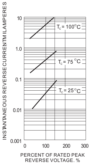
Fig.3-TYPICAL REVERSE CHARACTERISTIC
