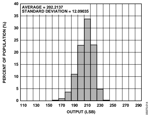
Figure 14. X-Axis Self-Test at 25^\circ\text{C} , V_{CC} = 5\text{ V}
