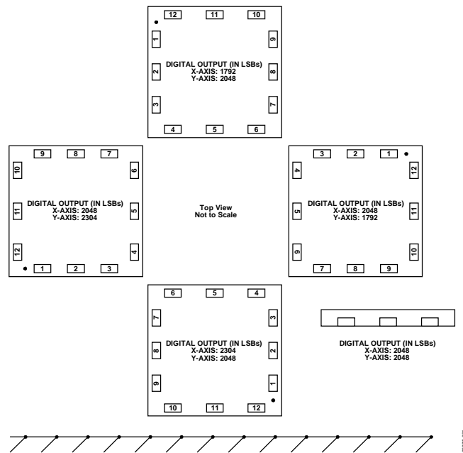
Figure 23. Output Response vs. Orientation
