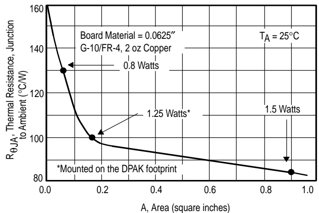
Figure 7. Thermal Resistance versus Collector Pad Area for the SOT-223 Package (Typical)
