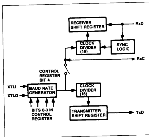
Figure 3. Transmitter/Receiver Clock Circuits
