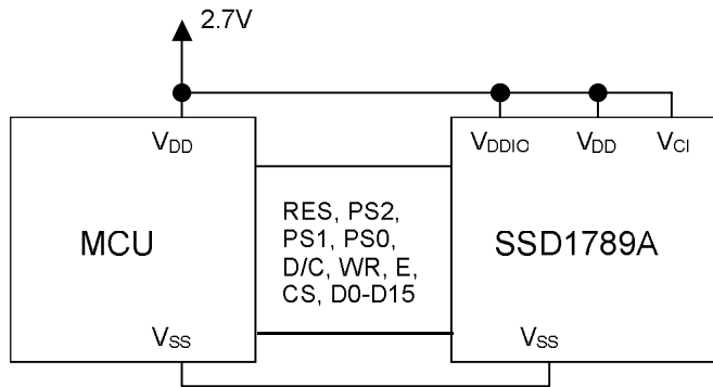
Figure 26 - V_{DD} , V_{DDIO} , V_{CI} connection example
