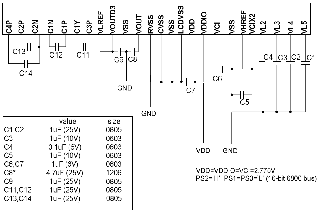
Figure 25 - Application example
