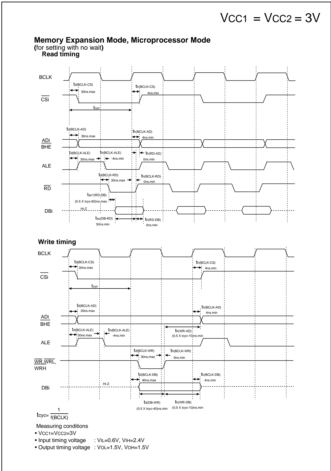
Figure 5.16 Timing Diagram (4)
