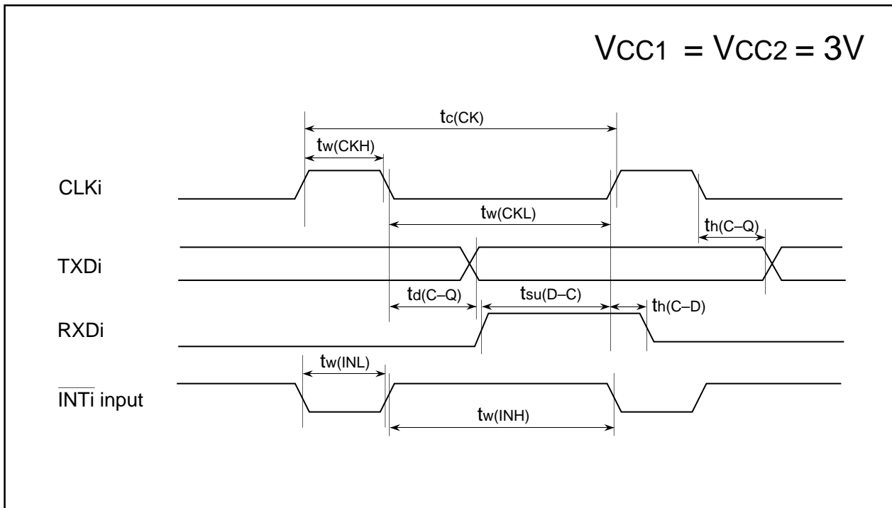
Figure 5.14 Timing Diagram (2)
