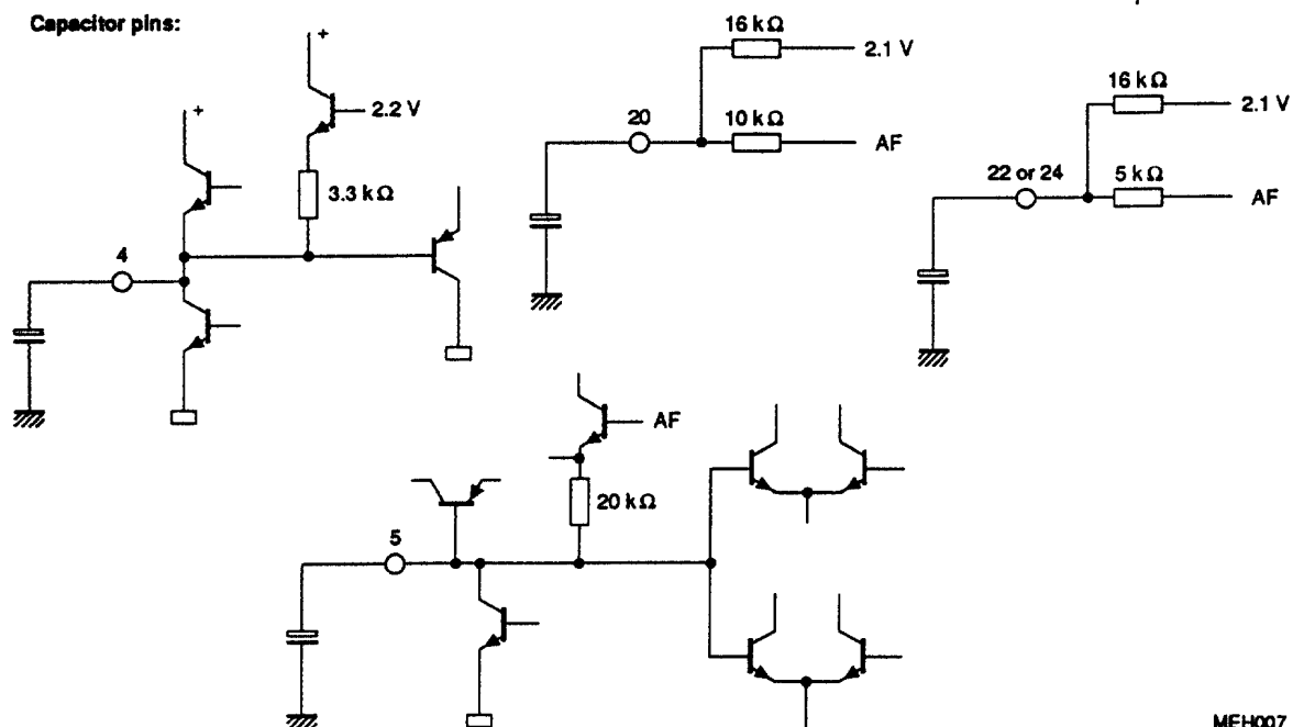
Fig.7 Internal circuits (continued from Fig.6).
