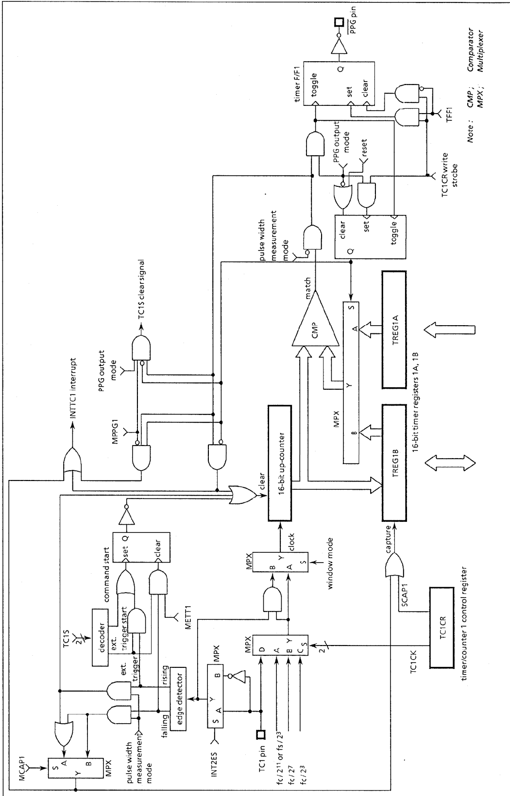
Figure 2-13. Timer/Counter 1
