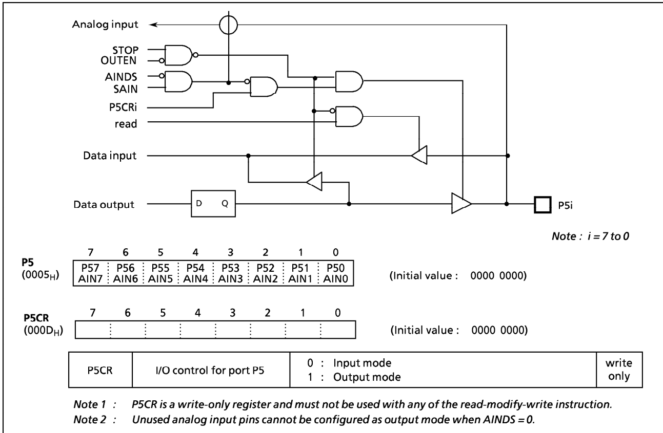
Figure 2-7. Port P5
