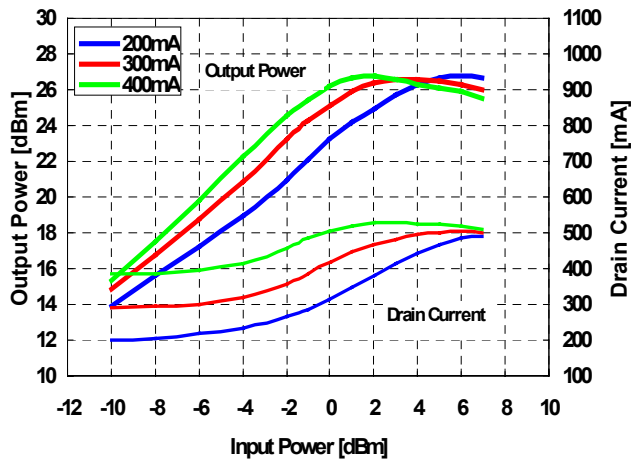
Output Power, Drain Current vs. Input Power by Drain Current @f=12GHz, VDD=6V
