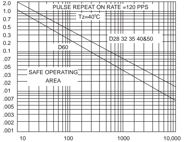
FIG.2-REPETITIVE PEAK ON-STATE CURRENT VS PULSE DURATION
