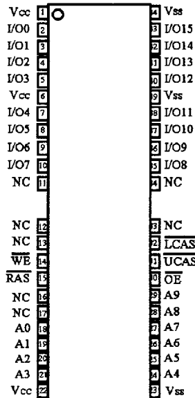
44 (50) TSOP II
