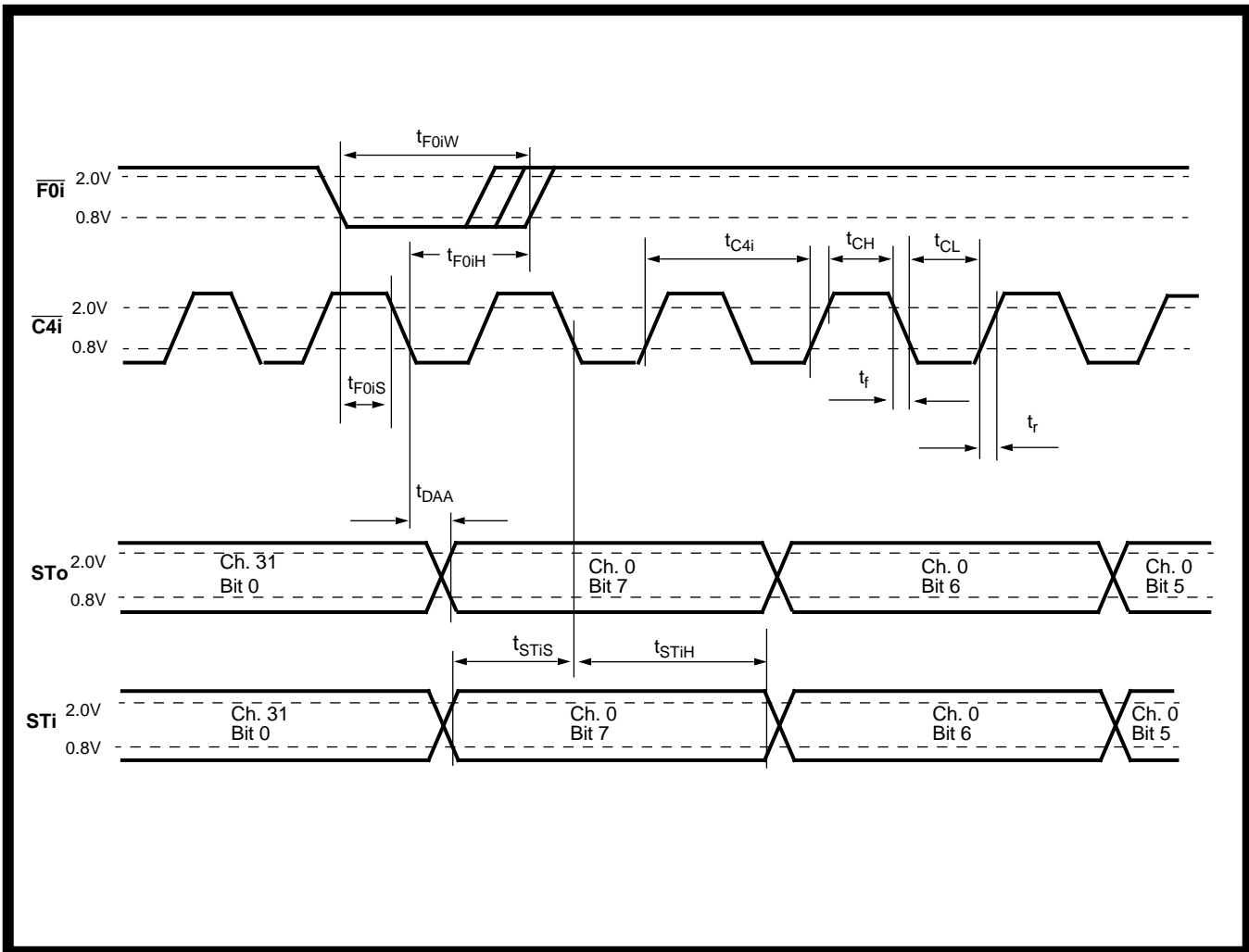
Figure 7 - ST-BUS Timing
