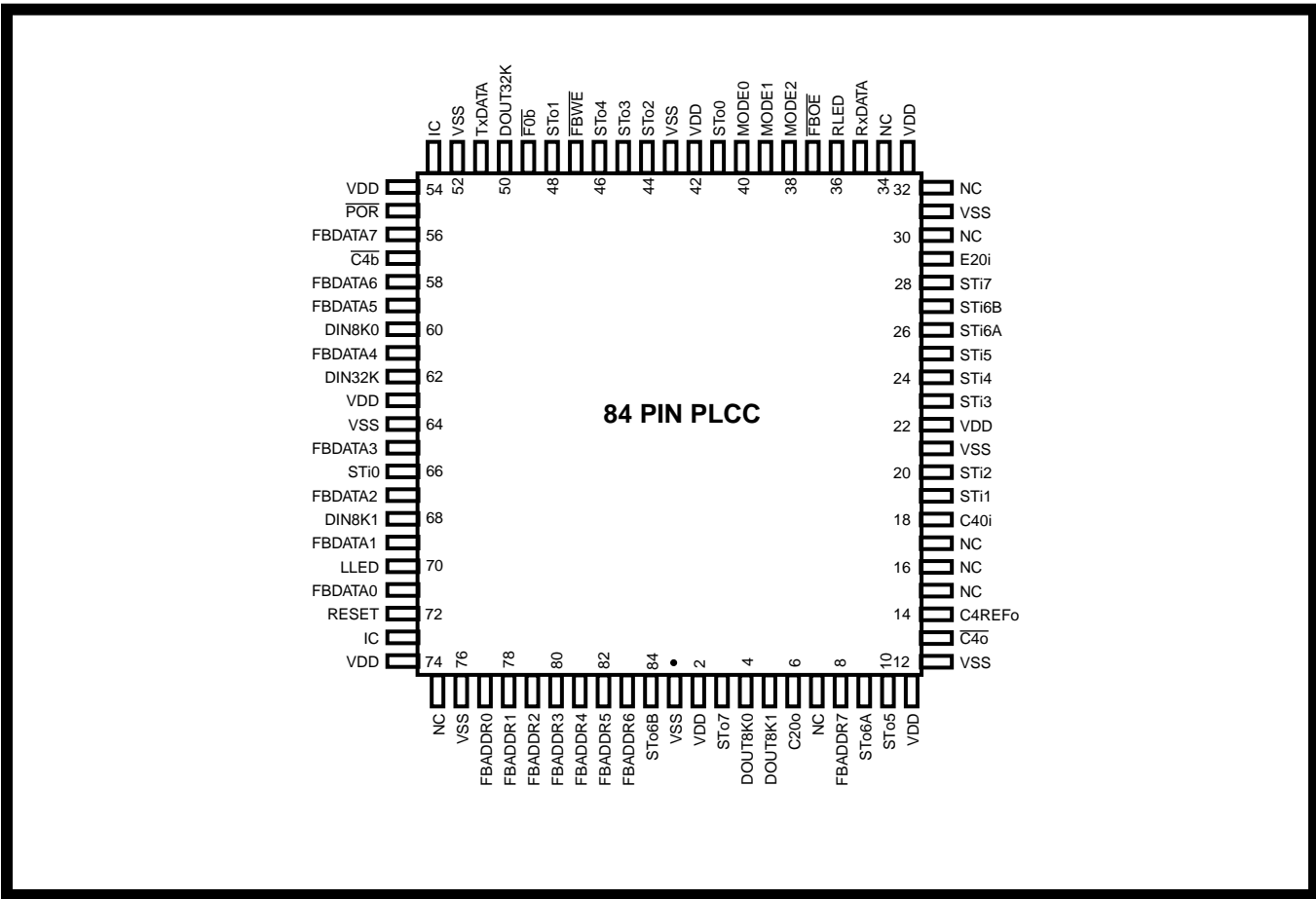
Figure 2 - Pin Connections
