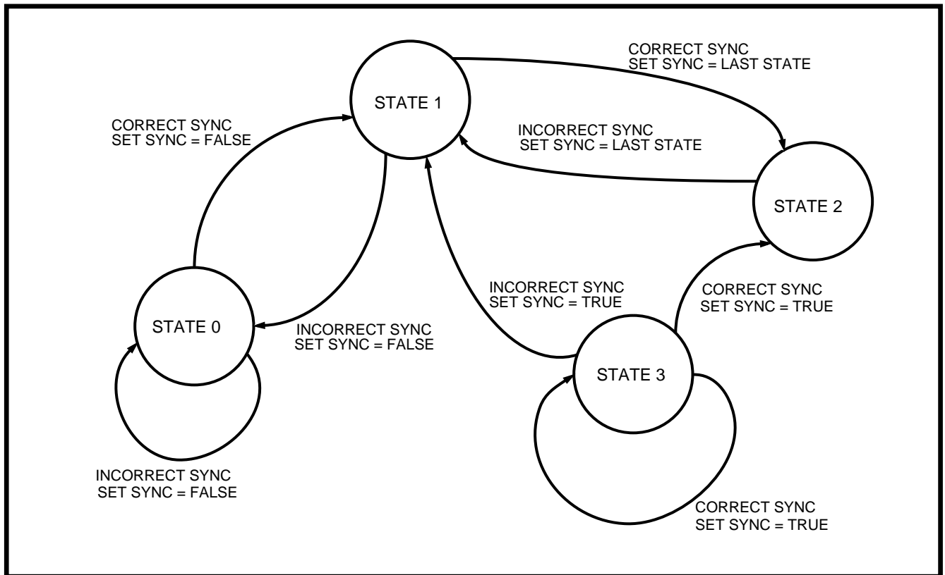
Figure 5 - State Diagram
