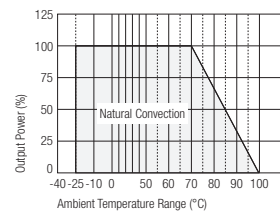
RP10-4805SE-M2
