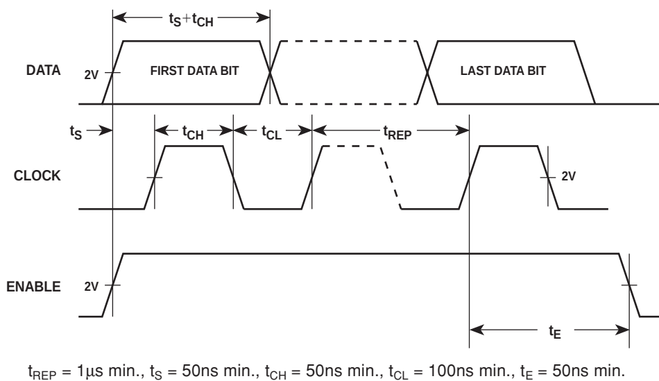
Fig. 5 Data and clock timing requirements
