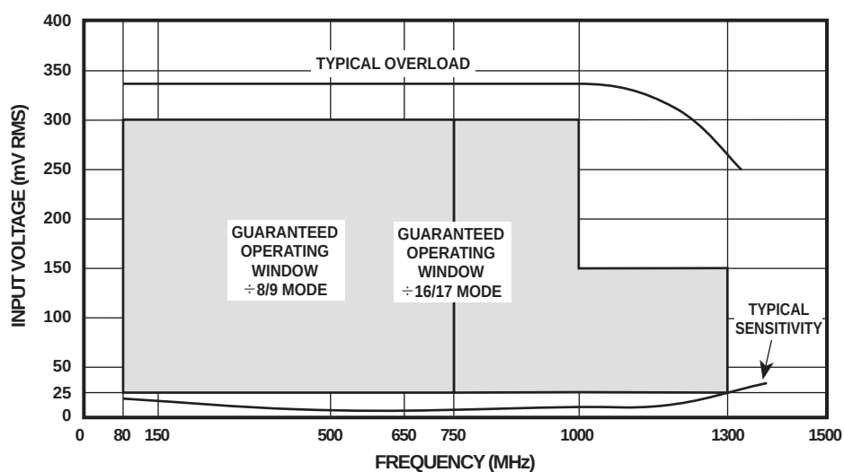
Fig. 4 Typical input characteristics and input drive requirements for SP8861
