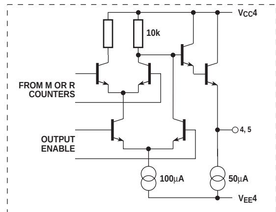
Fig. 8h F_{PD} and F_{REF} outputs
