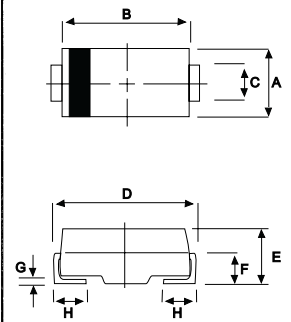
DO-214AA(SMB)
