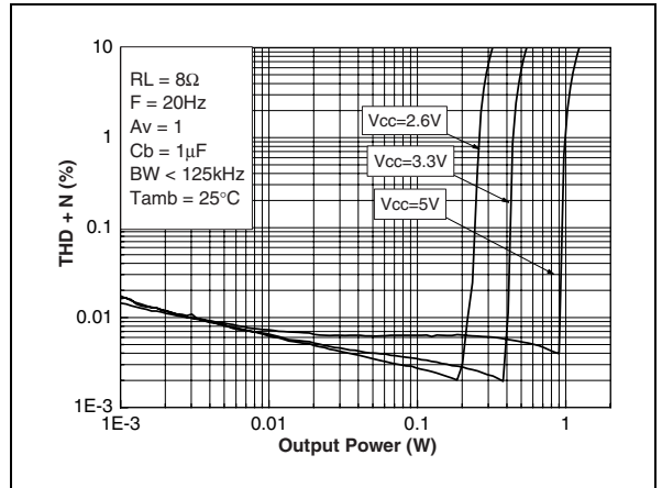
Figure 42. THD+N vs. output power
