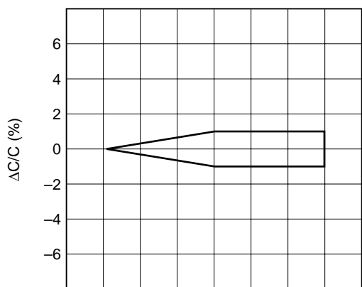
Rapid change of temperature (-55°C to +125°C, n = 50)
