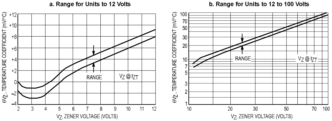
Figure 2. Temperature Coefficients
