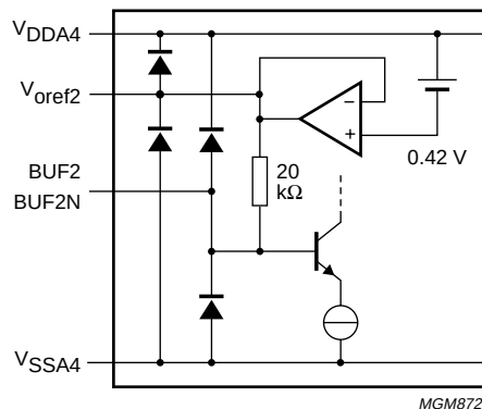
Fig.11 ADC2 buffer input and V_{\text{oref2}} output.
