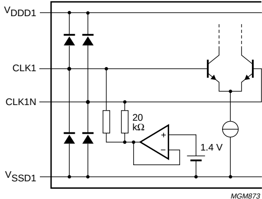
Fig.12 ADC1 clock buffer input.
