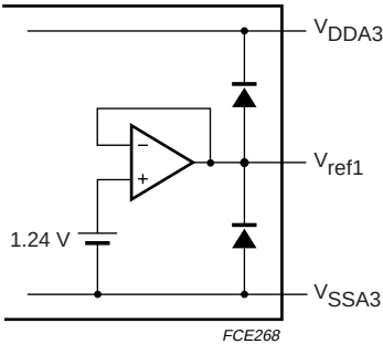
Fig.21 V_{ref1} output.
