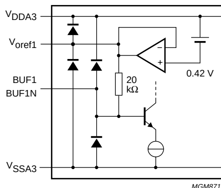
Fig.10 ADC1 buffer input and V_{\text{oref1}} output.
