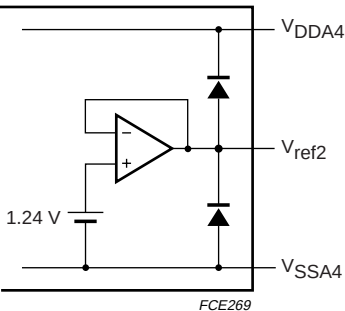
Fig.22 V_{ref2} output.
