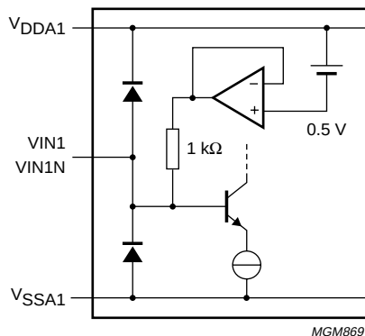
Fig.8 DPGA1 analog input.
