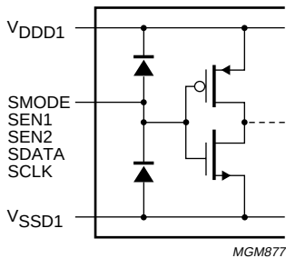
Fig.16 Serial Interface inputs.
