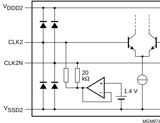
Fig.13 ADC2 clock buffer input.
