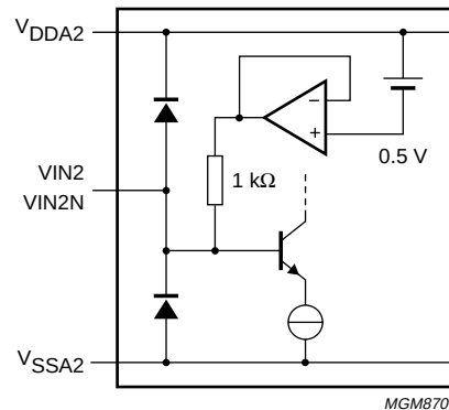
Fig.9 DPGA2 analog input.
