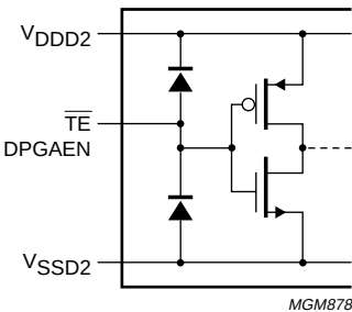
Fig.17 \overline{TE} and DPGAEN inputs.
