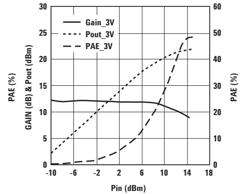
Figure 21. Small Signal Gain/Pout/PAE vs. Pin at V_{ds}=3V and Freq = 3.9 GHz.
