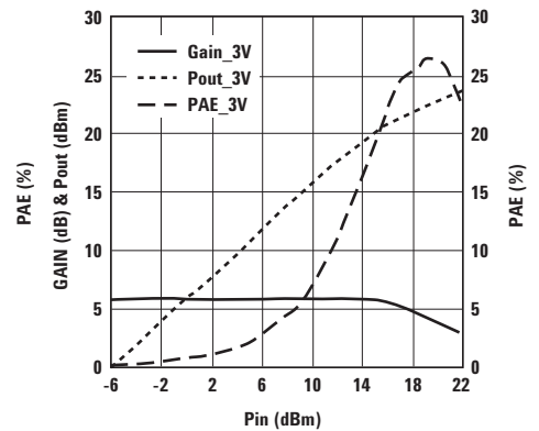
Figure 24. Small Signal Gain/Pout/PAE vs. Pin at V_{ds}=3V and Freq = 5.8 GHz.
