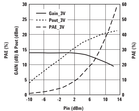
Figure 18. Small Signal Gain/Pout/PAE vs. Pin at V_{ds}=3V and Freq = 2 GHz.
