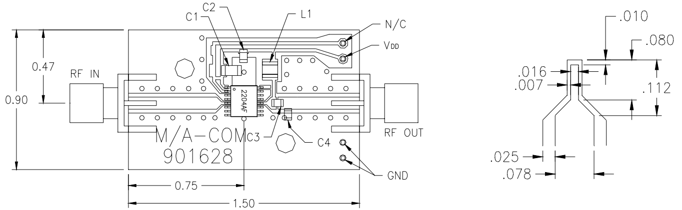
Top view 50Ω lead transition Figure 6. Component layout and printed circuit drawing for evaluation board
