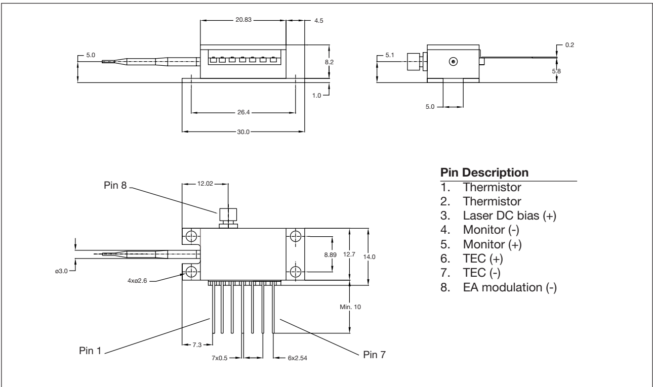
Figure 2. Pin description
